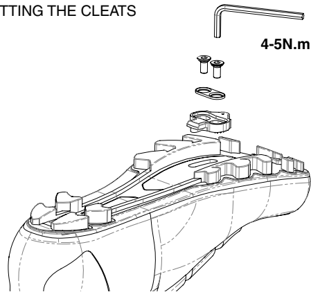
C / FITTING THE CLEATS
