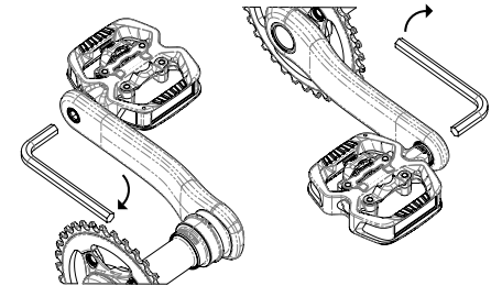
C / TIGHTENING THE PEDAL ON THE CRANK ARM
