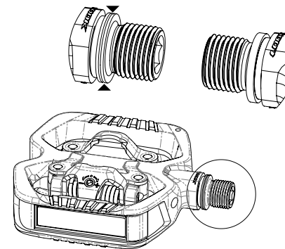
E / IDENTIFYING THE RIGHT AND LEFT PEDALS
